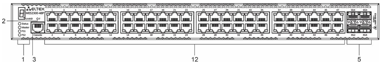
Figure 10 – MES2300-48P front panel
