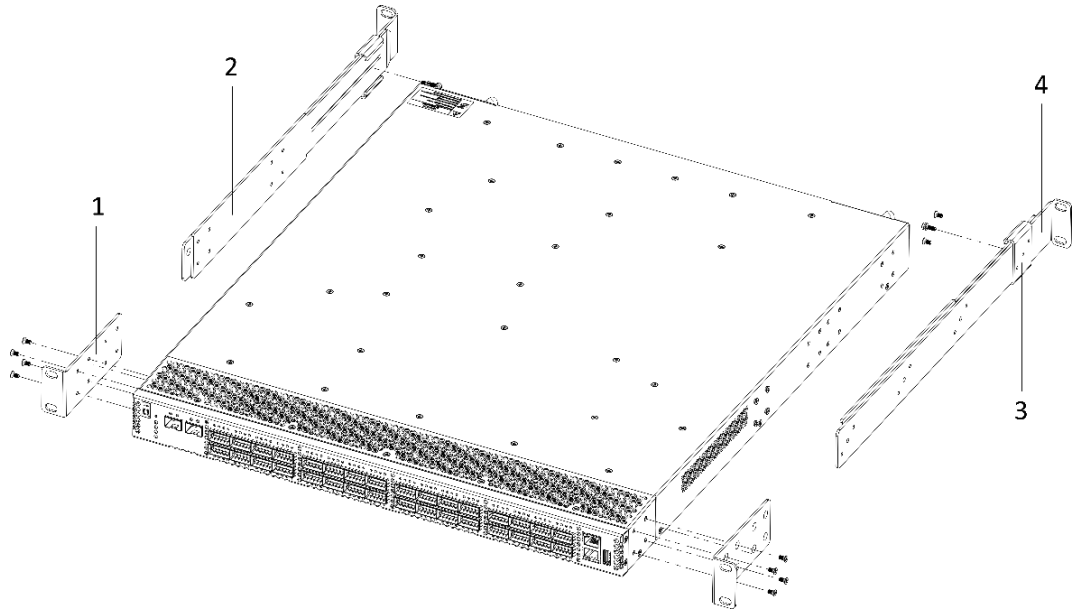
Figure 78 – Bracket mounting for MES5410-48, MES5500-32
