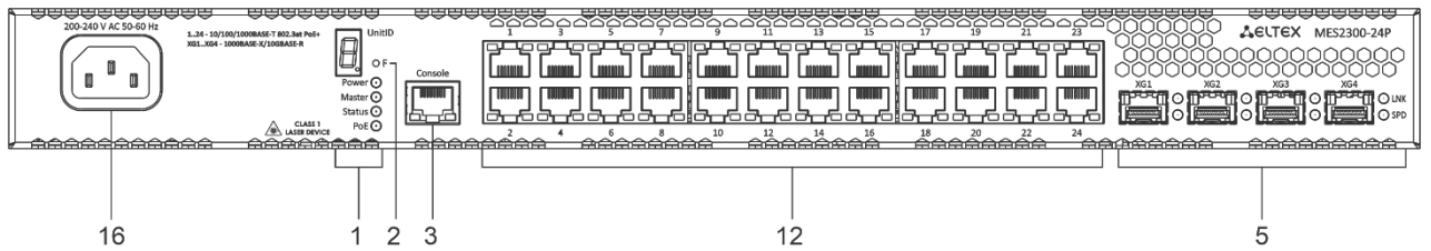
Figure 8 – MES2300-24P front panel
