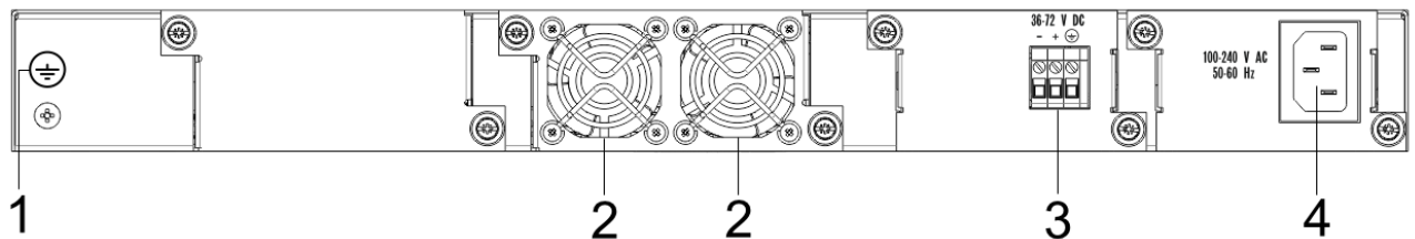
Figure 44 – MES5316A rear panel
