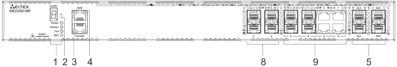
Figure 13 – MES3300-08F front panel
