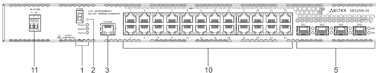
Figure 2 – MES2300-24 DC front panel
