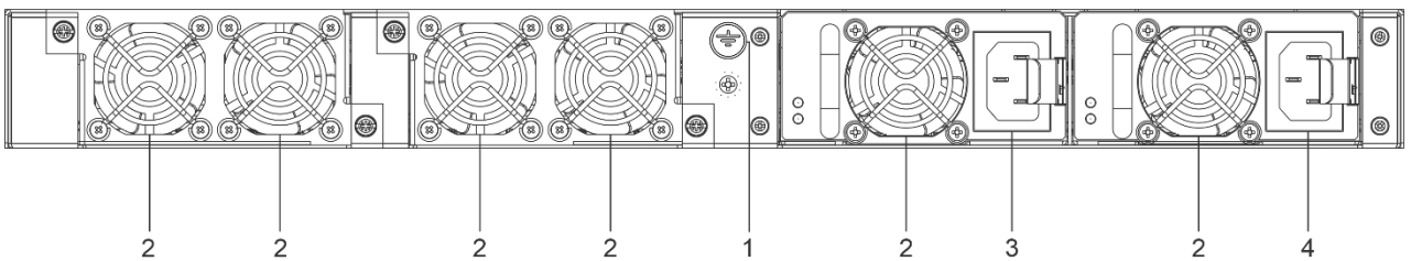
Figure 35 – MES2300-48P rear panel
