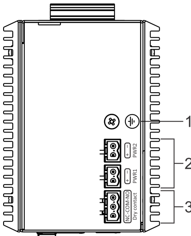
Figure 29 – MES3500I-08P and MES3500I-10P top panel
