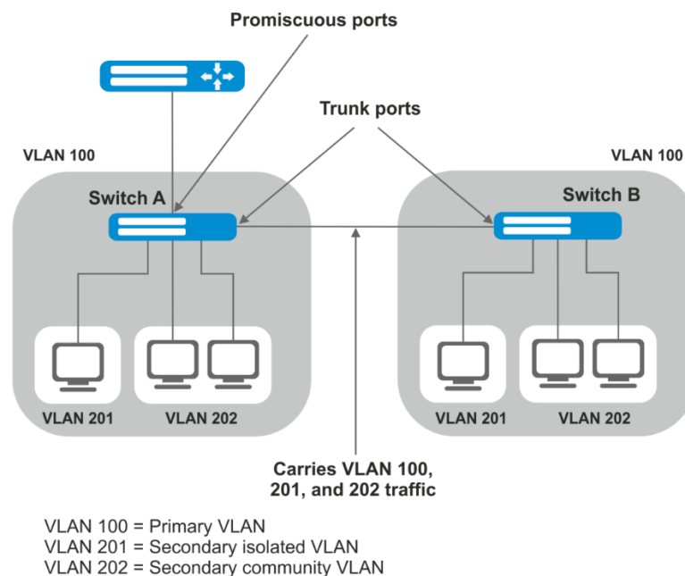
Figure 87 – Example of Private VLAN technology work
