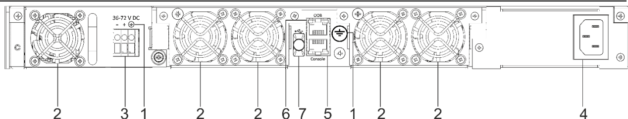
Figure 47 – MES5400-48 rear panel
