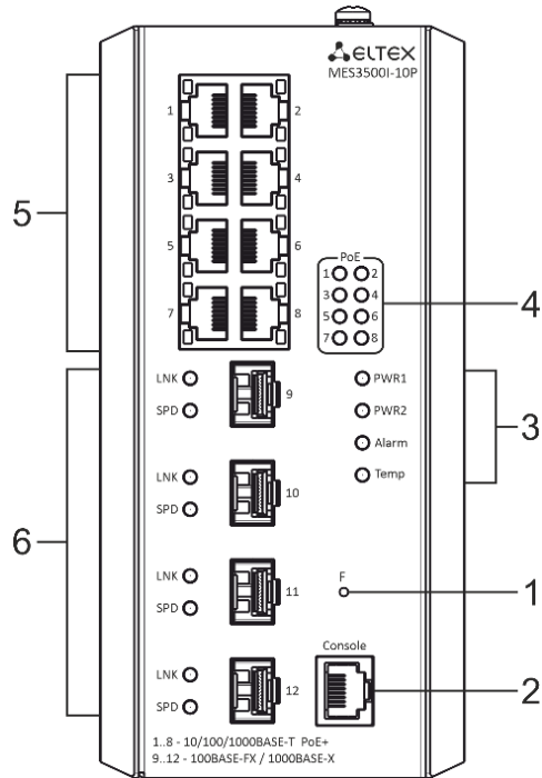
Figure 28 – MES3500I-10P front panel
