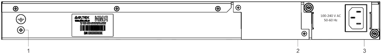
Figure 34 – MES2300DI-28 rear panel
