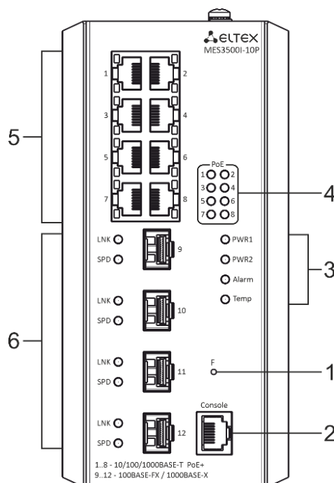
Figure 27 – MES3500I-08P front panel
