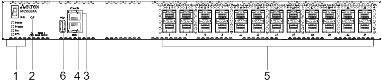
Figure 20 – MES5324A front panel
