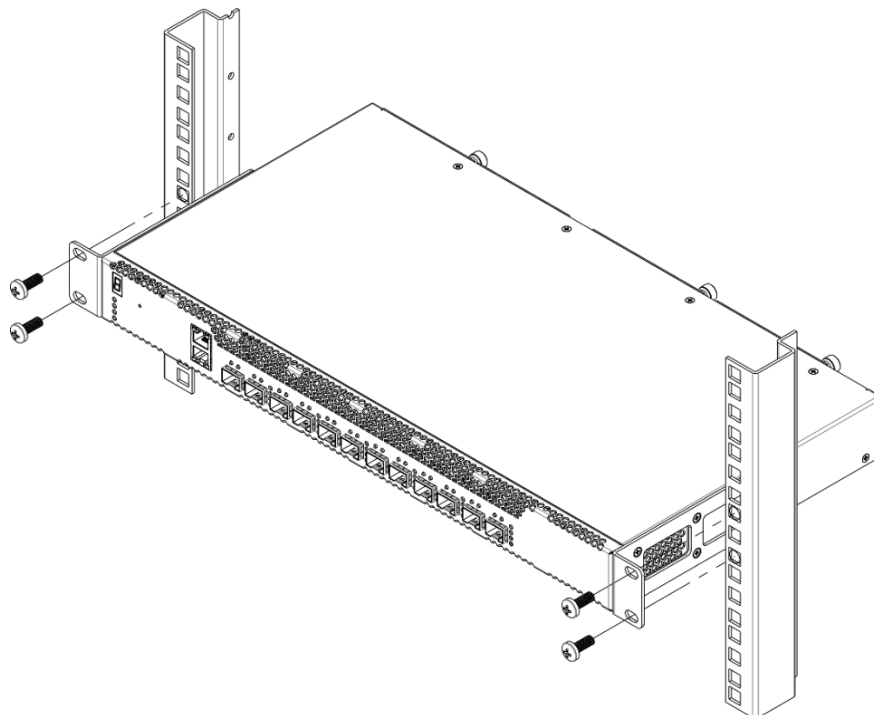
Figure 79 – Device rack mounting
