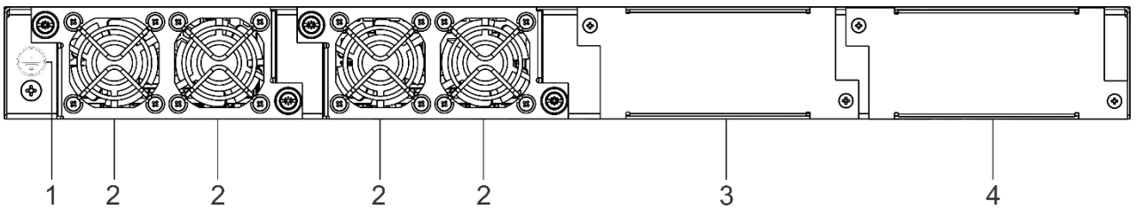
Figure 33 – MES2300D-24P rear panel
