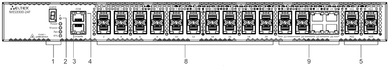
Figure 15 – MES3300-24F front panel
