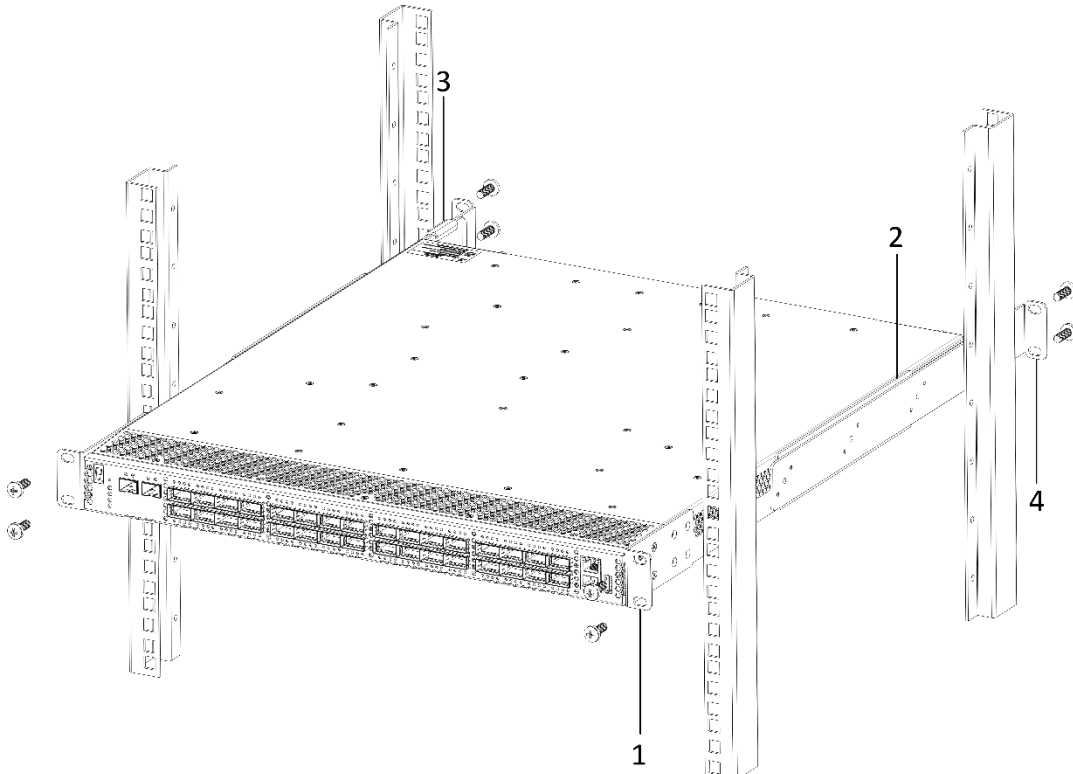
Figure 80 – MES5500-32 rack mounting
