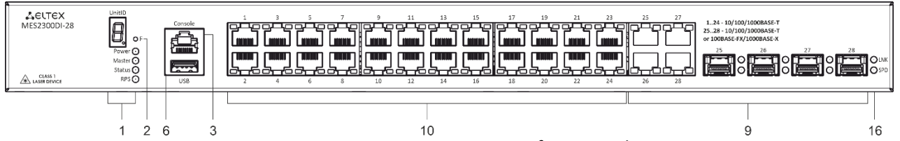
Figure 6 – MES2300DI-28 front panel
