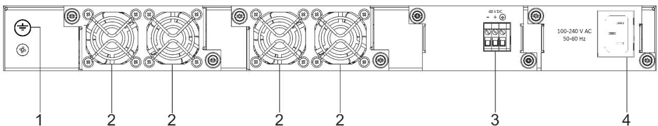
Figure 46 – MES5400-24 rear panel
