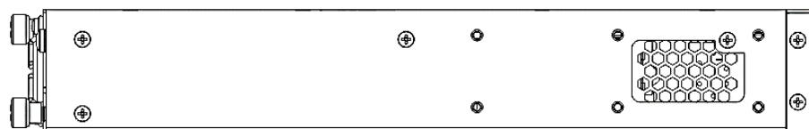
Figure 63 — MES5316A, MES5324A, MES5332A left side panel layout
