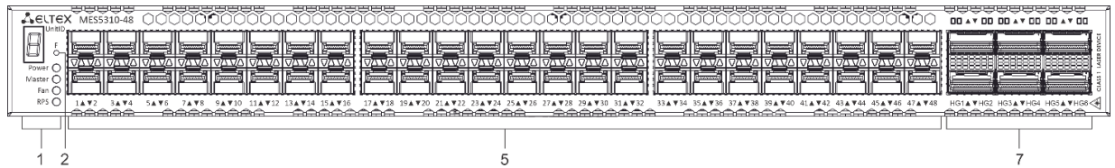
Figure 22 – MES5310-48 front panel
