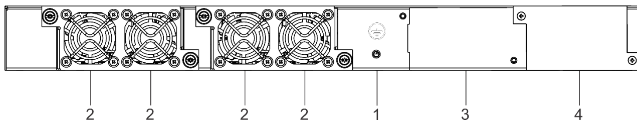
Figure 39 – MES3300-16F rear panel
