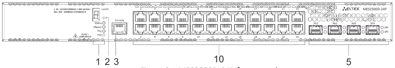
Figure 9 – MES2300D-24P front panel
