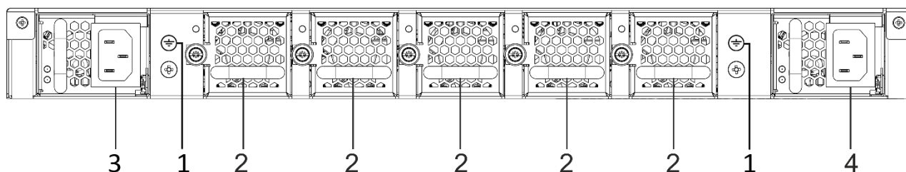
Figure 49 – MES5500-32 rear panel
