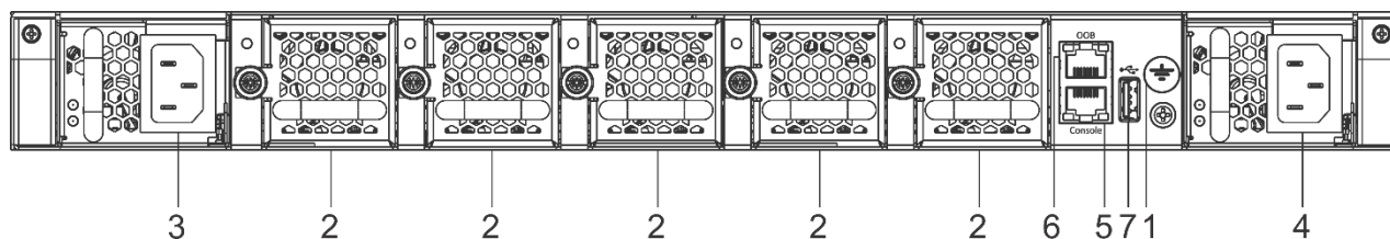
Figure 48 – MES5410-48 rear panel
