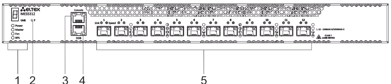
Figure 18 – MES5312 front panel
