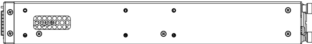
Figure 68 – MES5400-24, MES5400-48 right side panel layout
