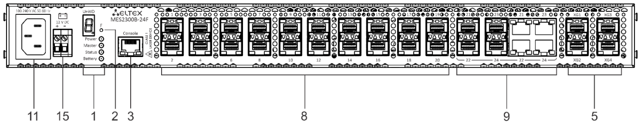
Figure 7 – MES2300B-24F front panel
