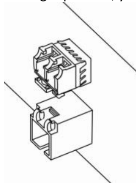
Figure 84 – Installed SFP transceivers
