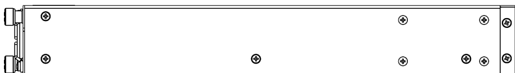
Figure 60 — MES3300-16F left side panel layout
