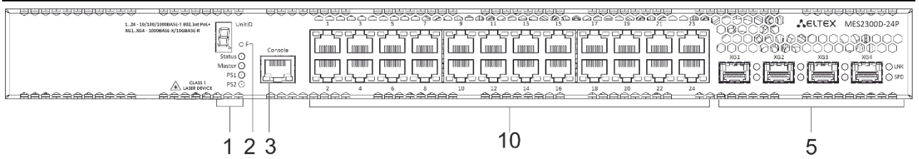
Figure 5 – MES2300D-24P front panel
