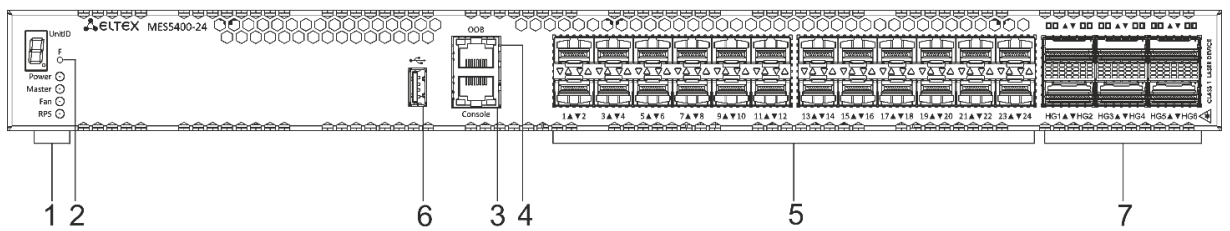
Figure 23 – MES5400-24 front panel
