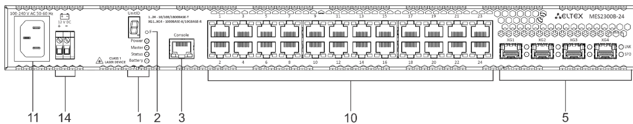
Figure 3 – MES2300B-24 front panel
