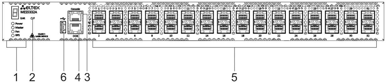
Figure 21 – MES5332A front panel
