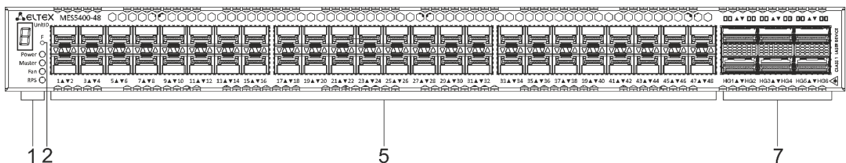
Figure 24 – MES5400-48 front panel
