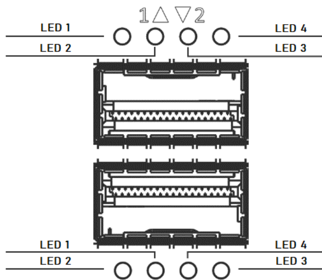
Figure 75 – QSFP+ and QSFP28 socket layout for MES5500-32
