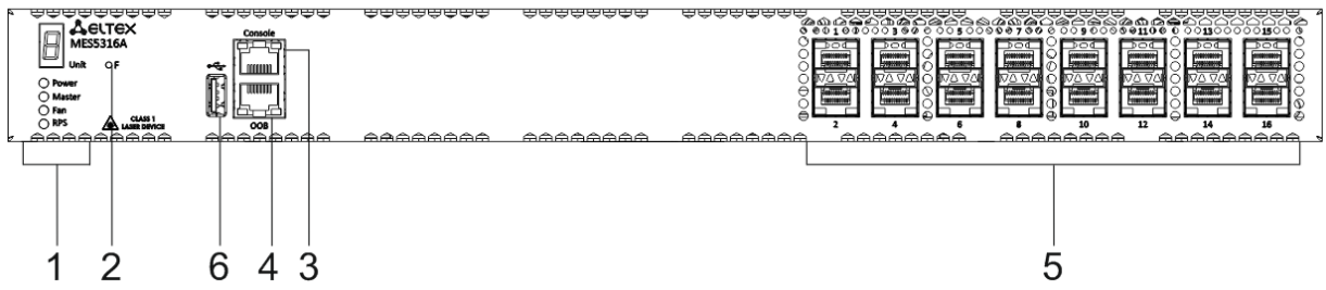
Figure 19 – MES5316A front panel
