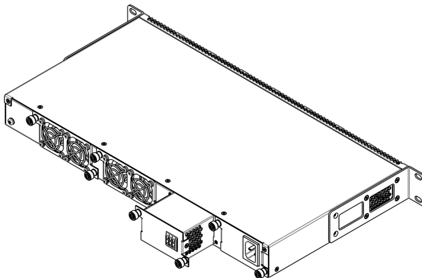
Figure 82 – Power module installation
