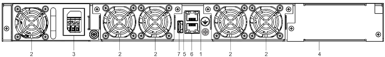
Figure 45 – MES5310-48 rear panel
