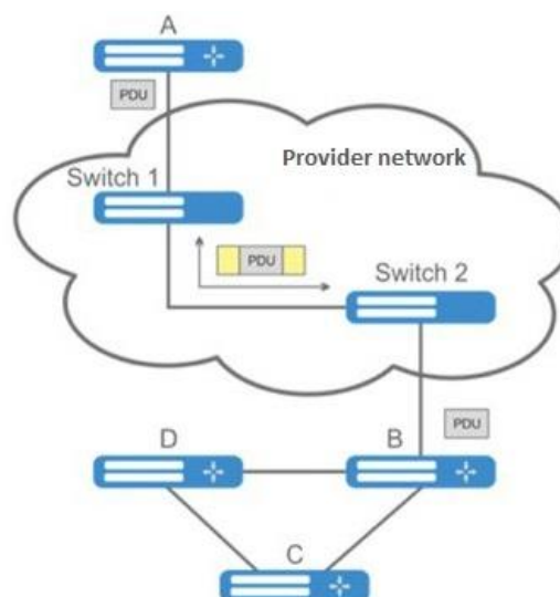
Figure 88 — L2PT function work example
