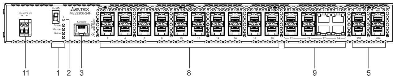
Figure 4 – MES2300-24F front panel
