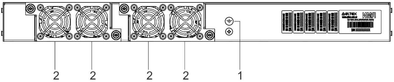
Figure 31 – MES2300-24F, MES2300B-24F rear panel
