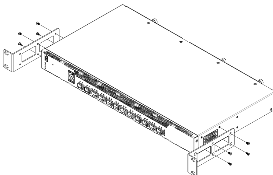
Figure 77 – Bracket mounting option No. 2
