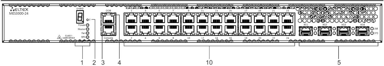
Figure 12 – MES3300-24 front panel
