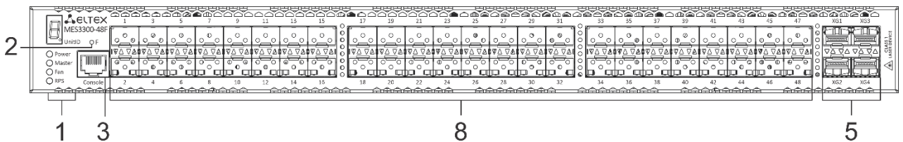
Figure 17 – MES3300-48F front panel
