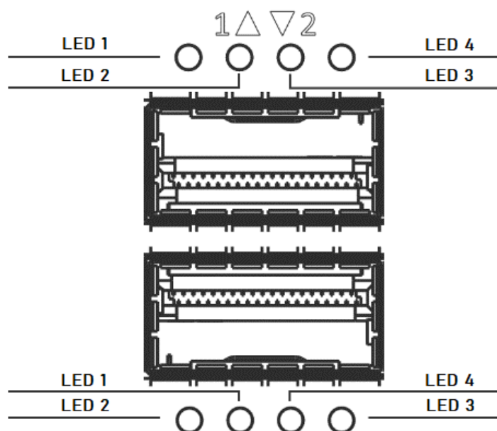
Figure 71 – QSFP+ and QSFP28 socket layout for MES5500-32
