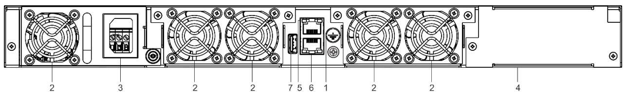
Figure 41 – MES5316A rear panel
