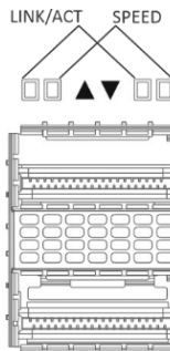
Figure 70 – QSFP+ and QSFP28 socket layout for MES5400-xx, MES5410-48
