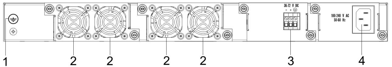
Figure 40 – MES5312, MES5324A, MES5332A rear panel
