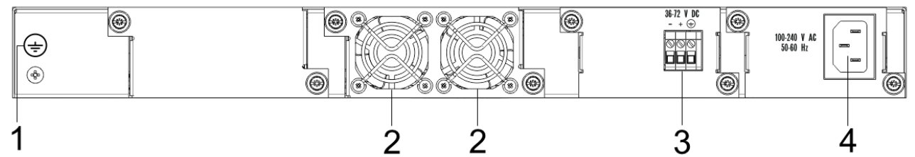
Figure 41 – MES5316A rear panel
