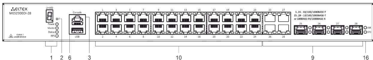
Figure 4 – MES2300DI-28 front panel
