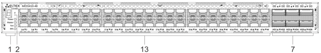
Figure 23 – MES5410-48 front panel
