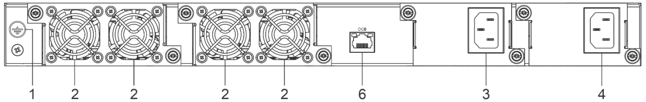
Figure 38 – MES3300-48, MES3300-48F rear panel
